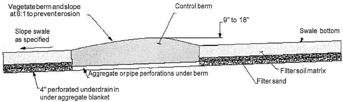
SWALE PROFILE
