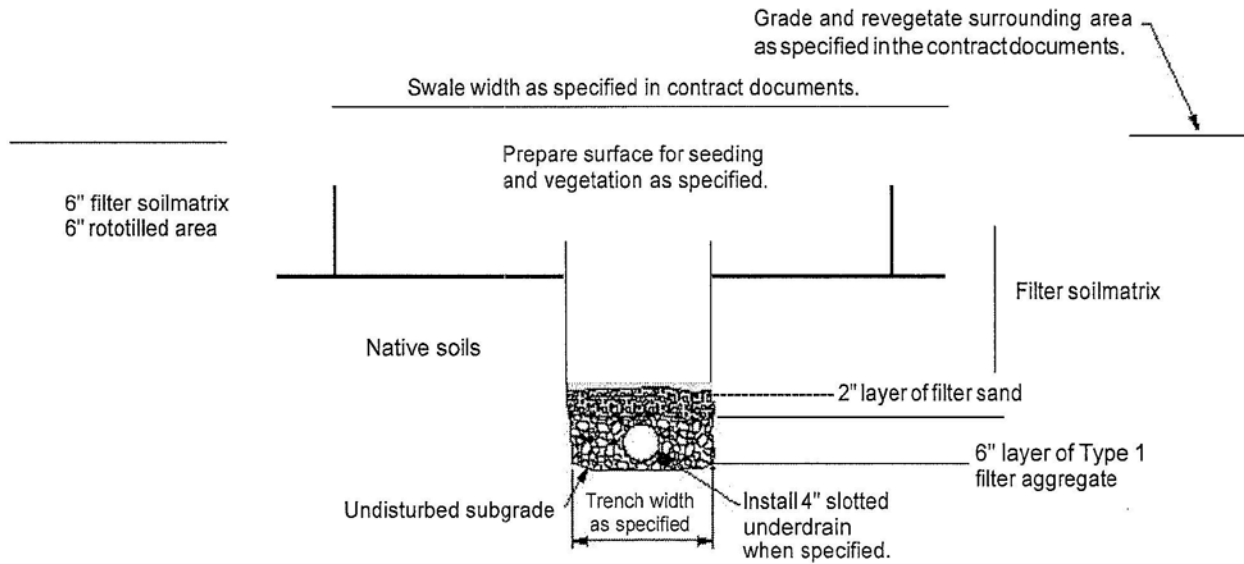
CROSS-SECTION
