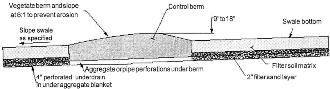
SWALE PROFILE
