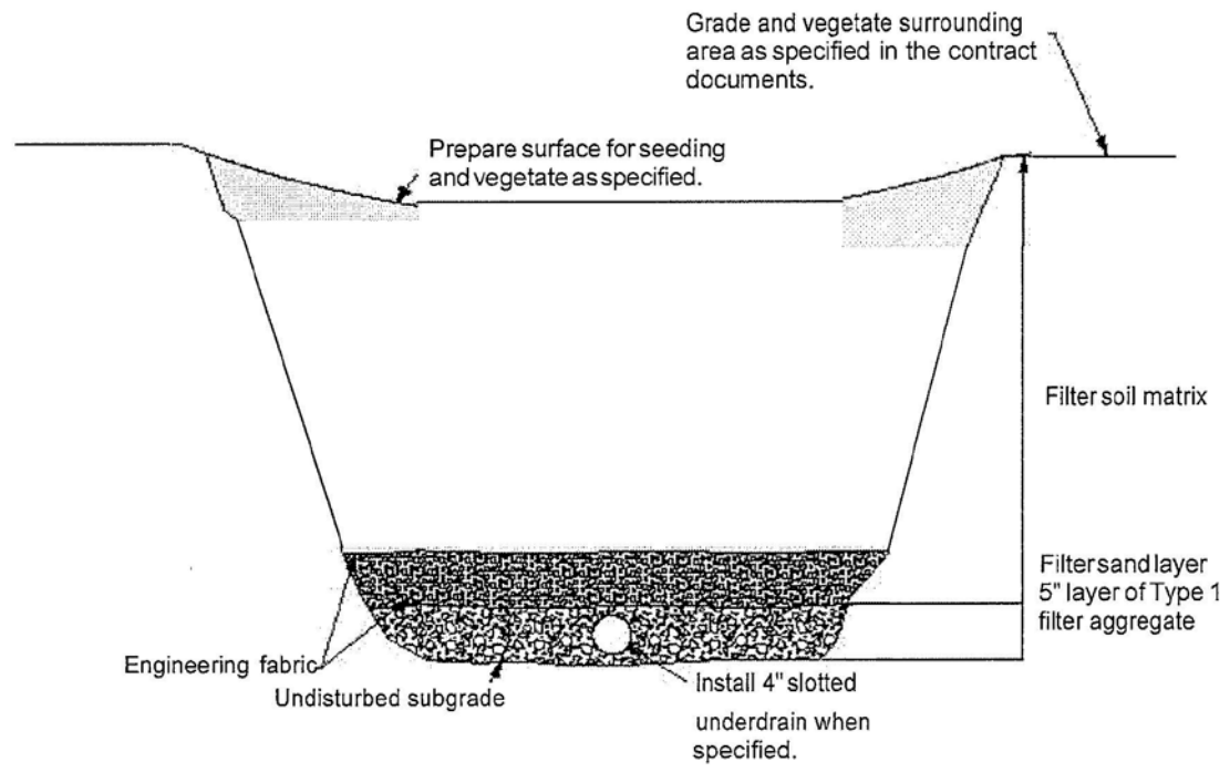
CROSS-SECTION
